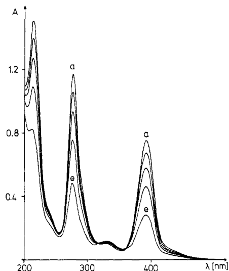
Figure 2. Spectral changes during the photolysis of aqueous 4.06 \times 10^{-5} M (\text{NH}_4)_2[\text{WS}_4] at (a) 0 and (e) 75-min irradiation time, with \lambda_{\text{irr}} > 200 nm and a 1-cm cell.
